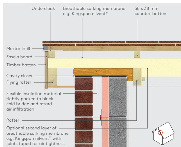
Figure 7c - Eaves detail
