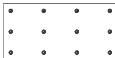
12 No. per board (1.2 x 0.6 m board - 16.66 fixings / m 2 ) (1.2 x 1.2 m board - 8.33 fixings / m 2 ) (2.4 x 1.2 m board - 4.16 fixings / m 2 )
