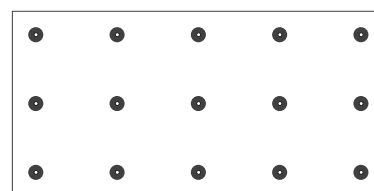
15 No. per board (1.2 x 0.6 m board - 20.83 fixings / m 2 ) (1.2 x 1.2 m board - 10.41 fixings / m 2 ) (2.4 x 1.2 m board - 5.20 fixings / m 2 )
